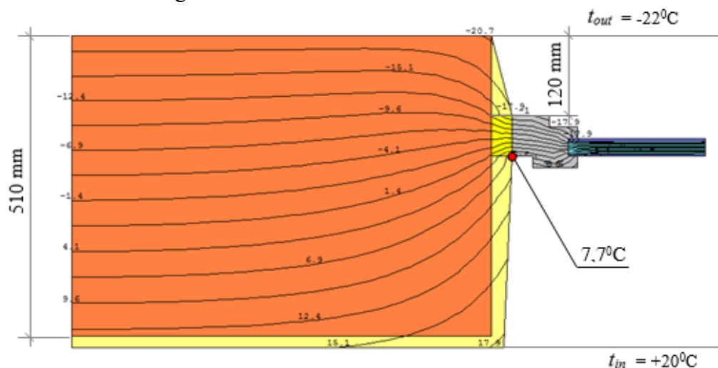
Figure 2 – Temperature distribution in the wall and in the window nodes area without a casing in a brick wall (the window is located at a distance of 120 mm from the facade surface of the wall). Source: developed by the authors
